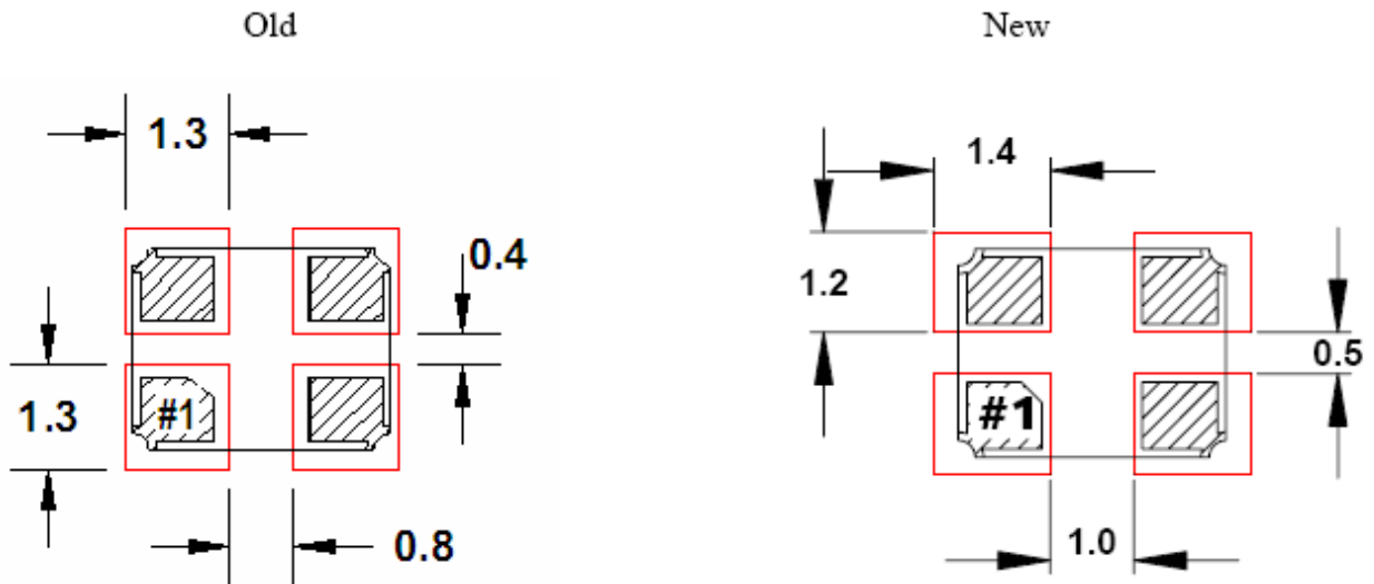
Top view of package superimposed on solder pad layout.
